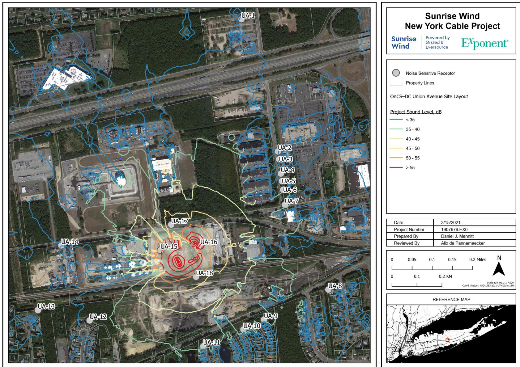
Revised Figure 19. OnCS-DC at the Union Avenue Site operational noise contours.
