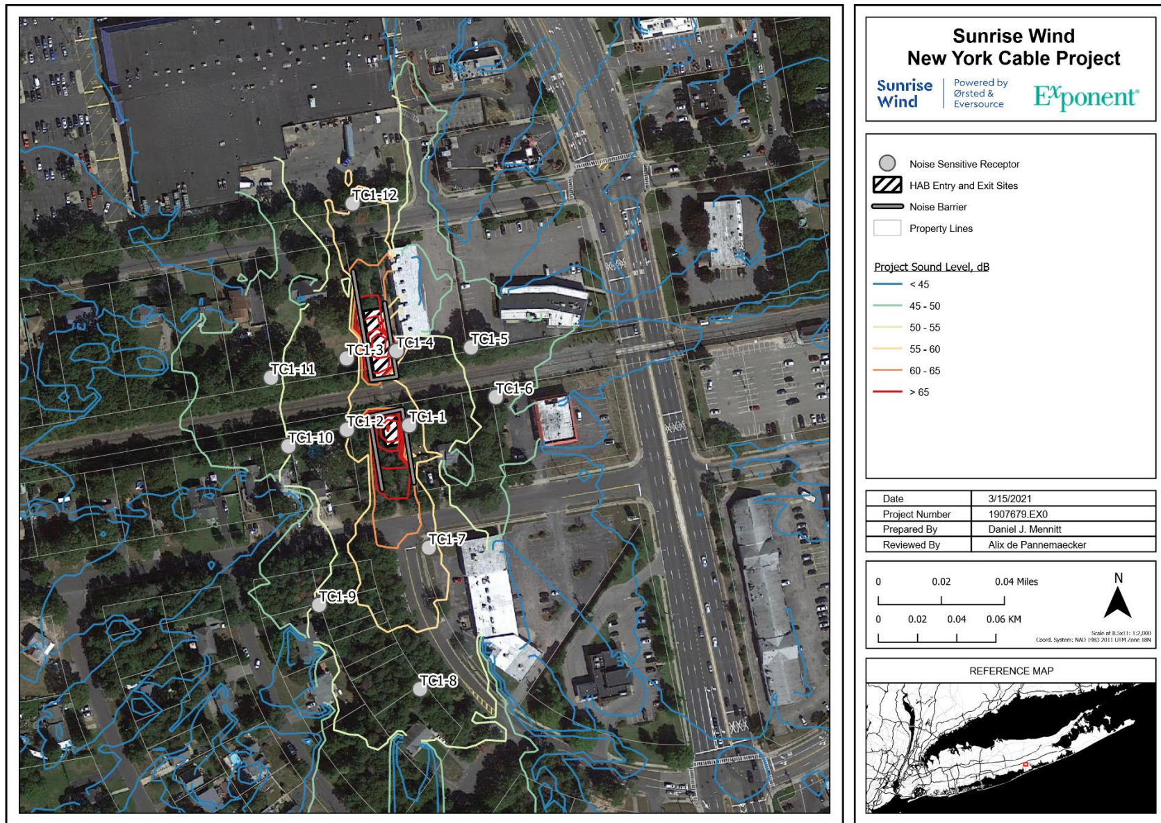
Revised Figure 13. TC1 HAB daytime construction noise contours.
