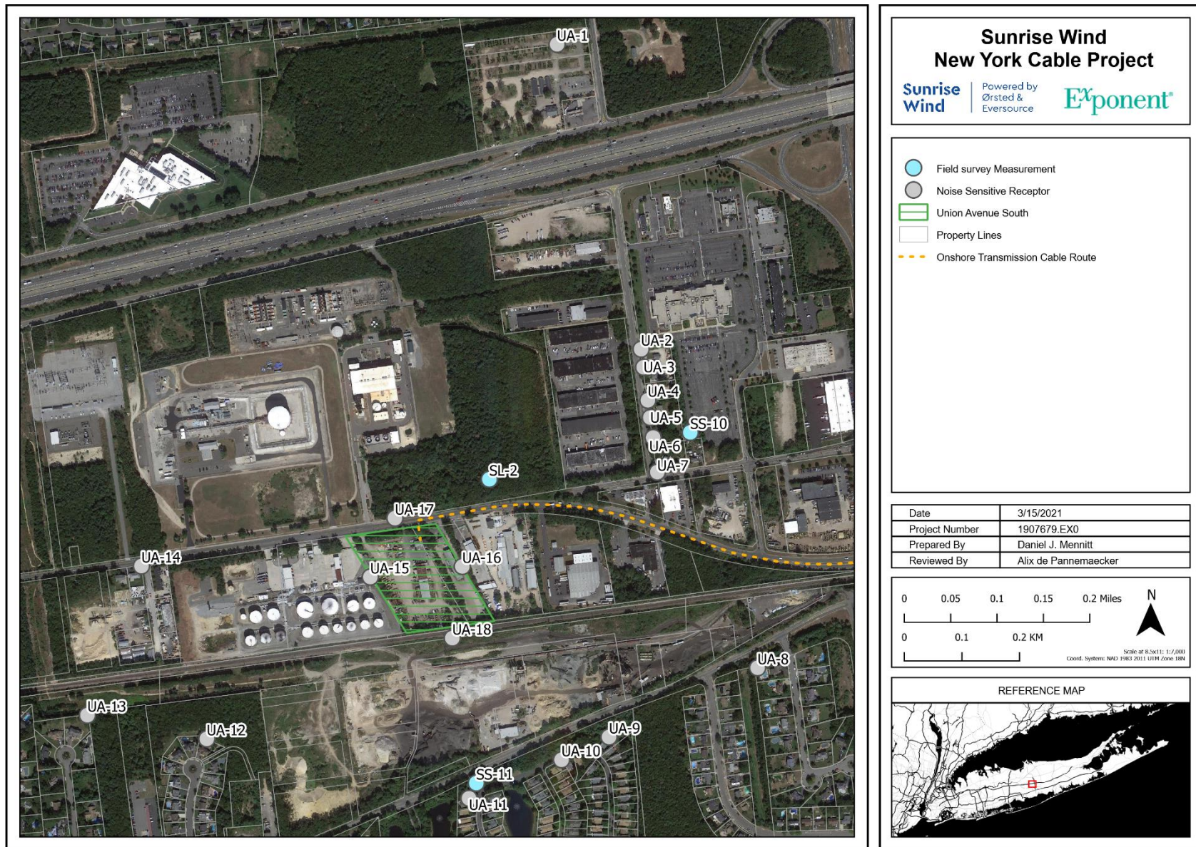
Revised Figure 4. Field survey measurement and NSR locations in the vicinity of the Union Avenue Site.
