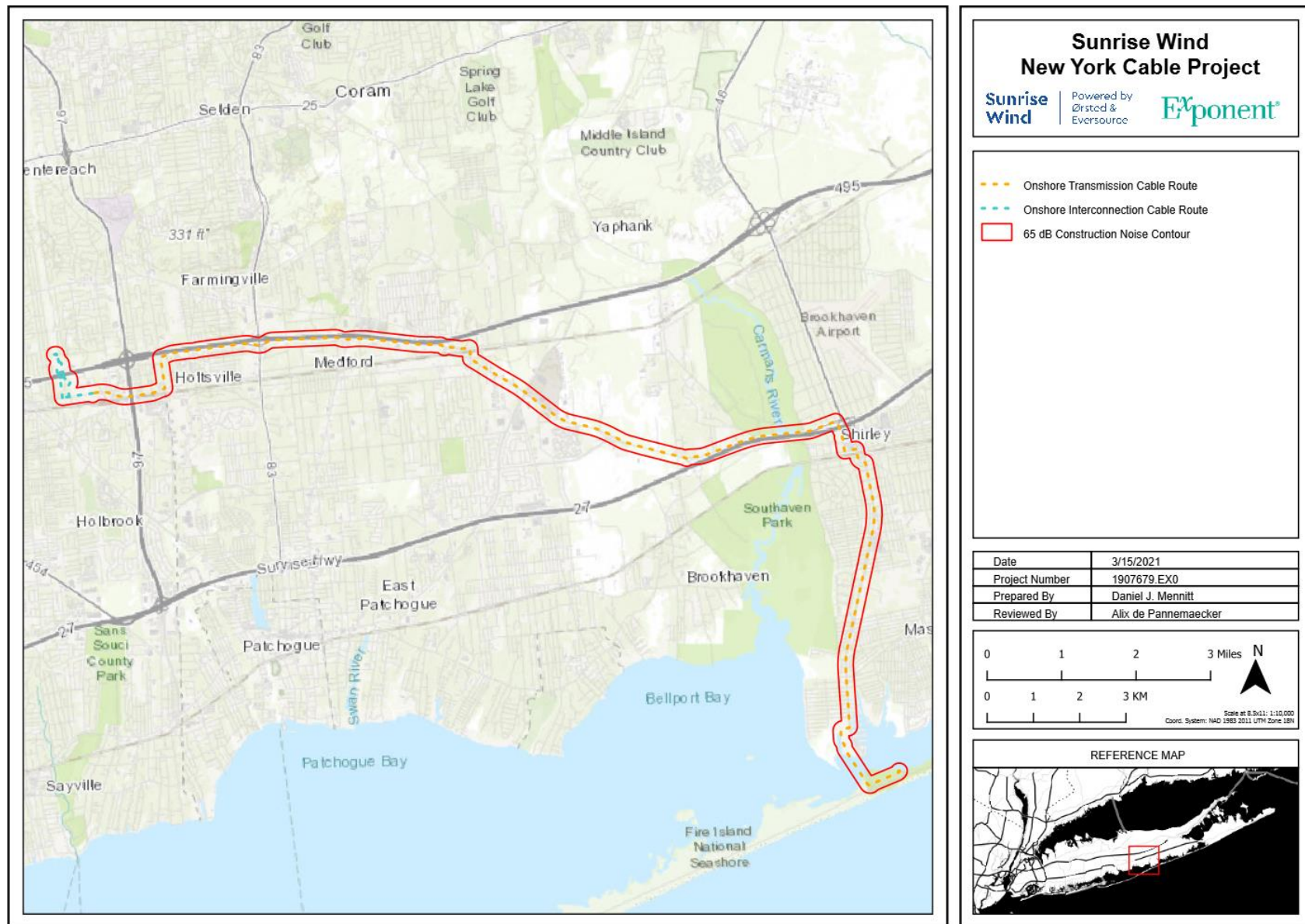
Revised Figure 18. Onshore cable routes and 65 dB construction noise contours.
