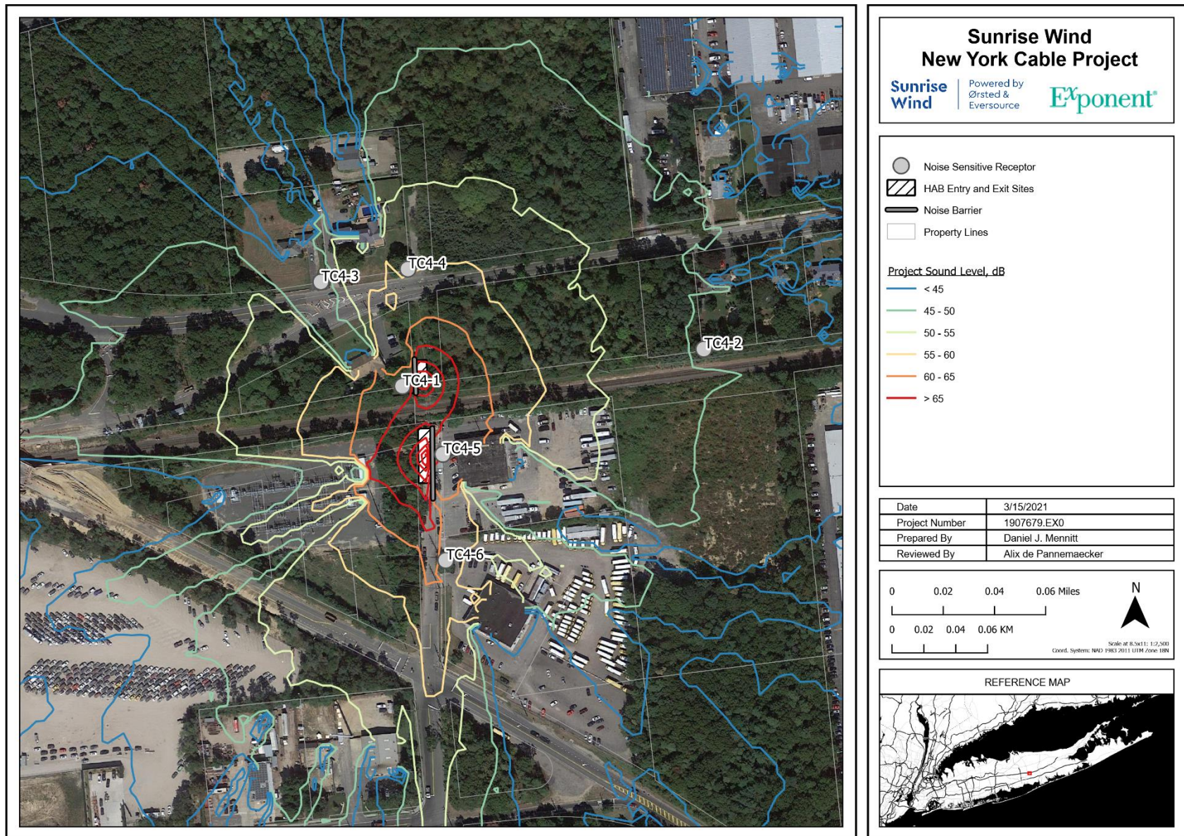
Revised Figure 16. TC4 HAB daytime construction noise contours.
