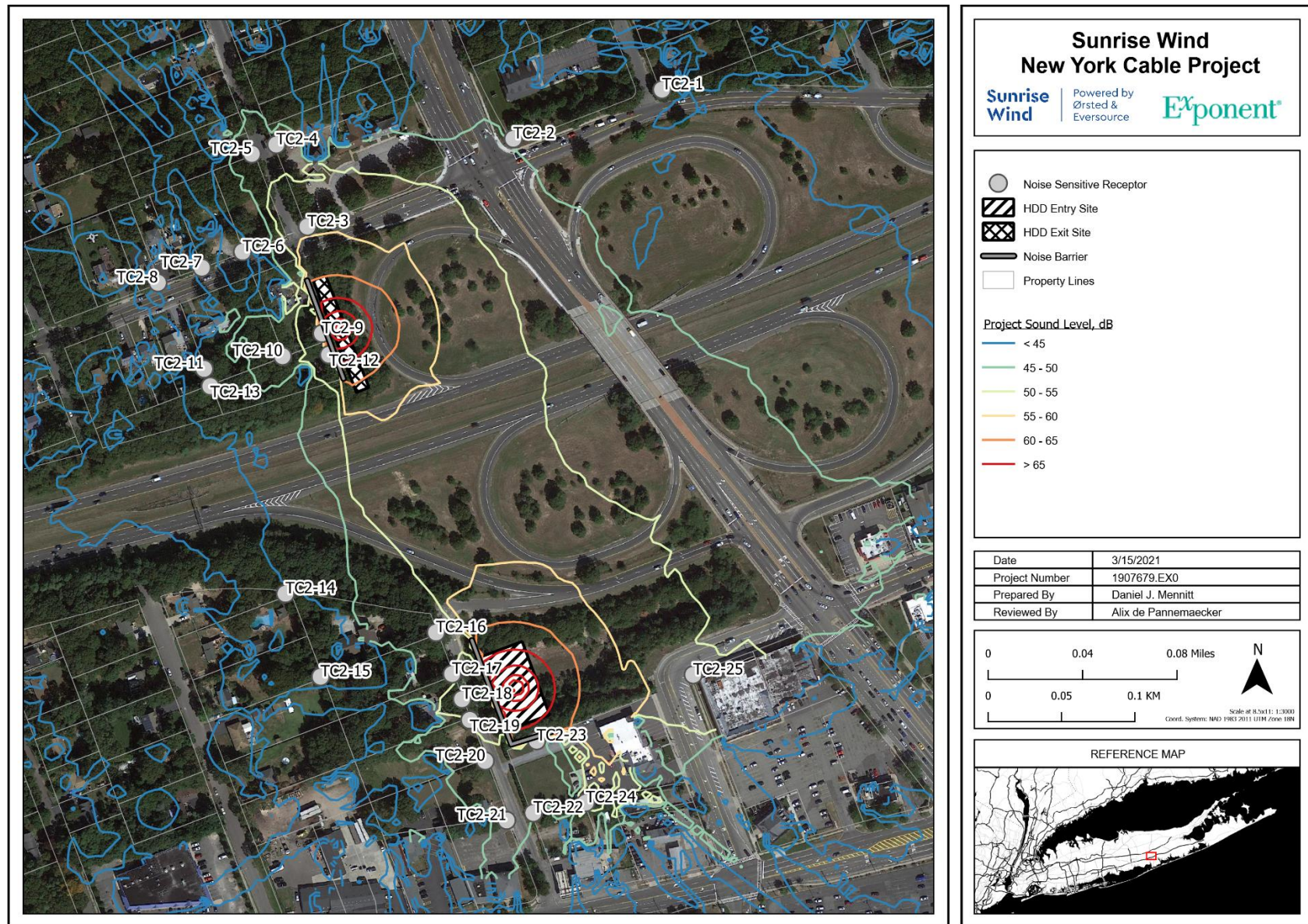
Revised Figure 14. TC2 HDD daytime construction noise contours.
