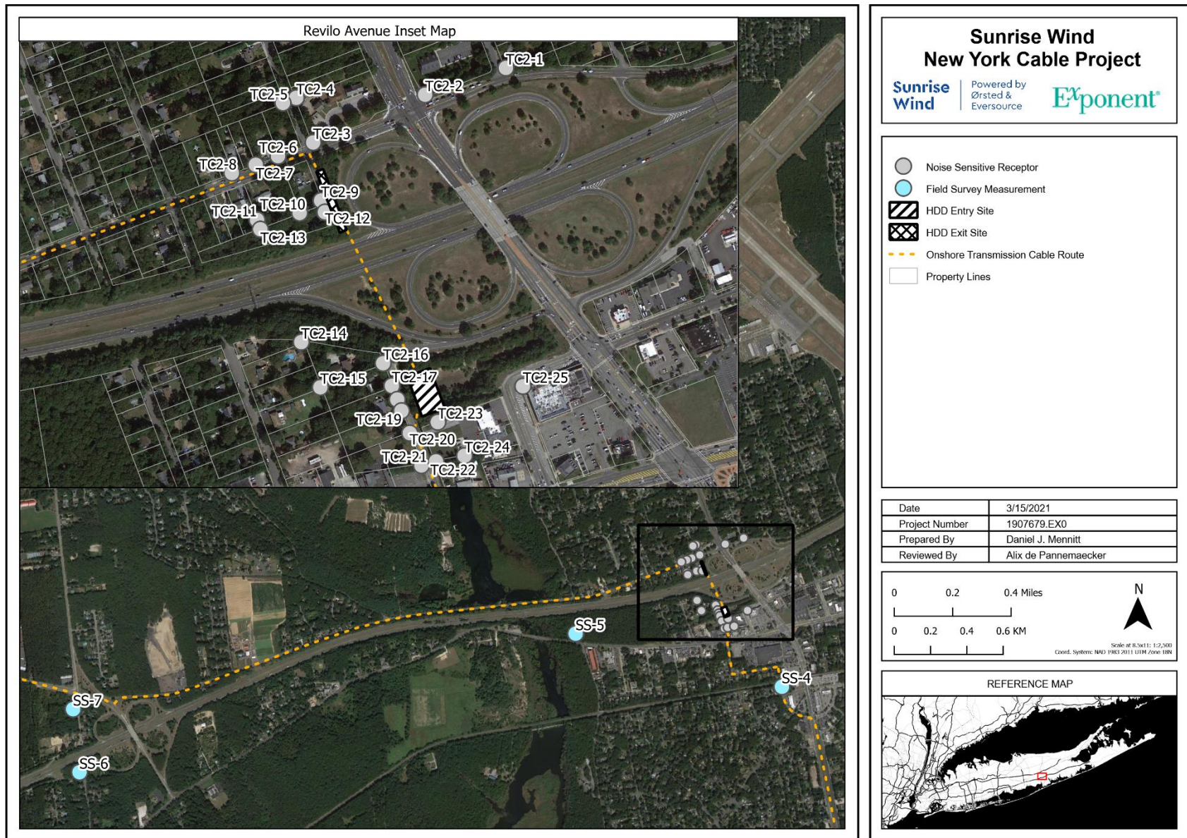
Revised Figure 7. Field survey measurement and NSR locations in the vicinity of TC2.
