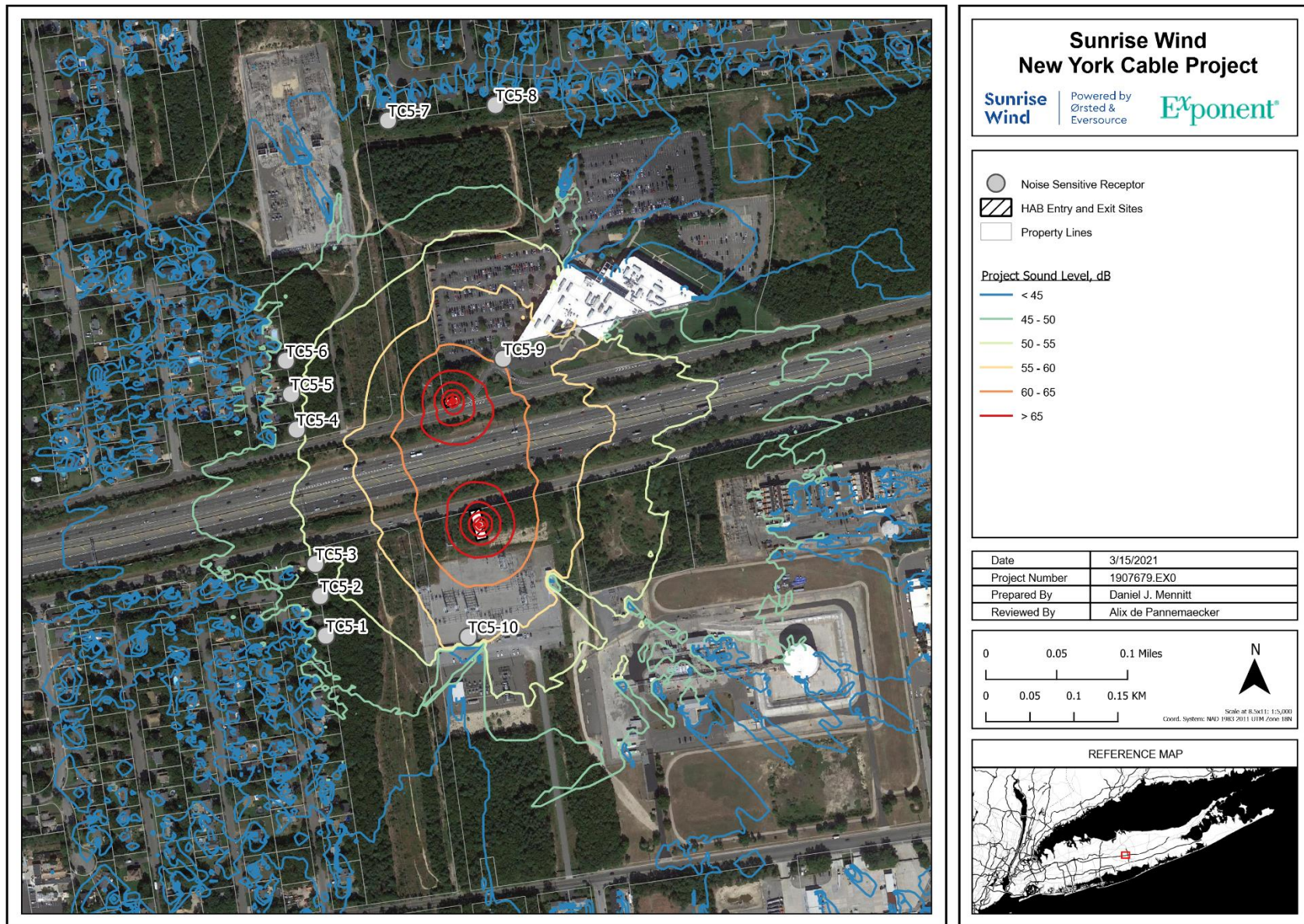
Revised Figure 17. TC5 HAB daytime construction noise contours.
