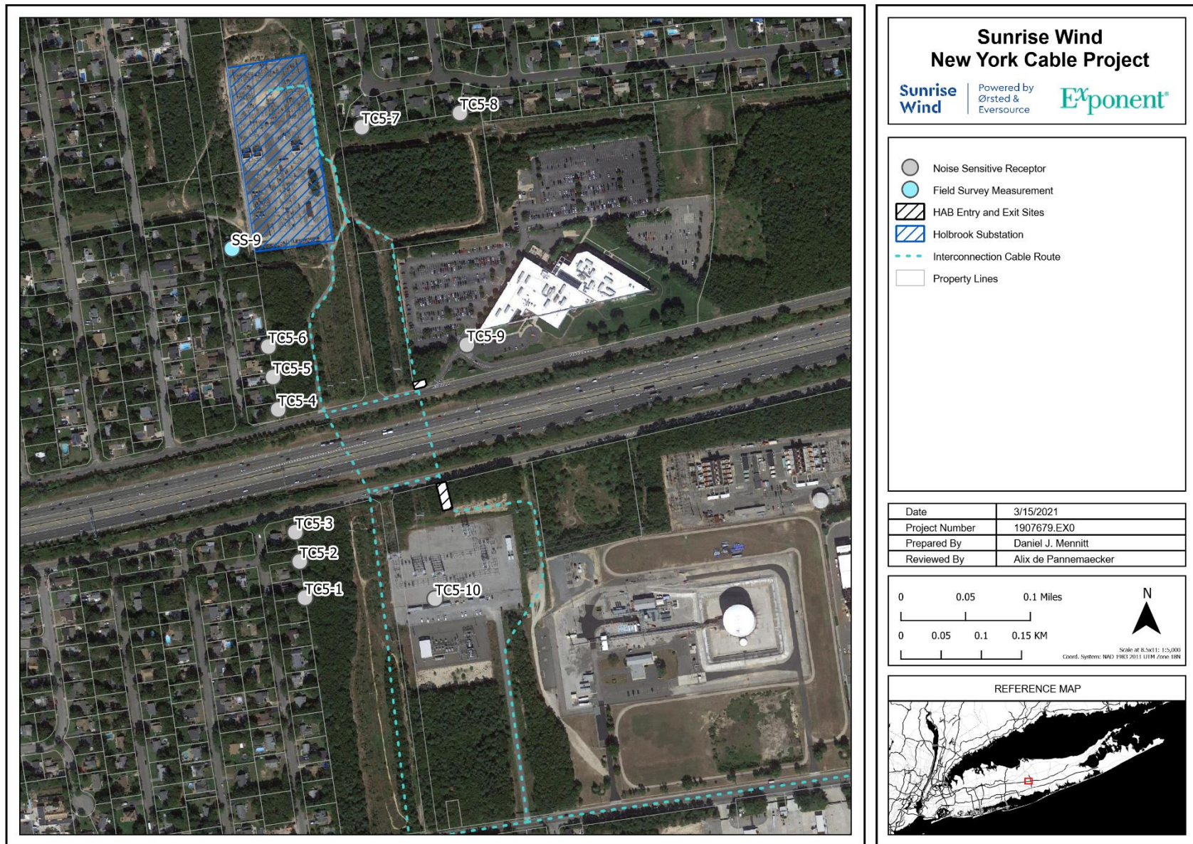
Revised Figure 10. Field survey measurement and NSR locations in the vicinity of TC5.
