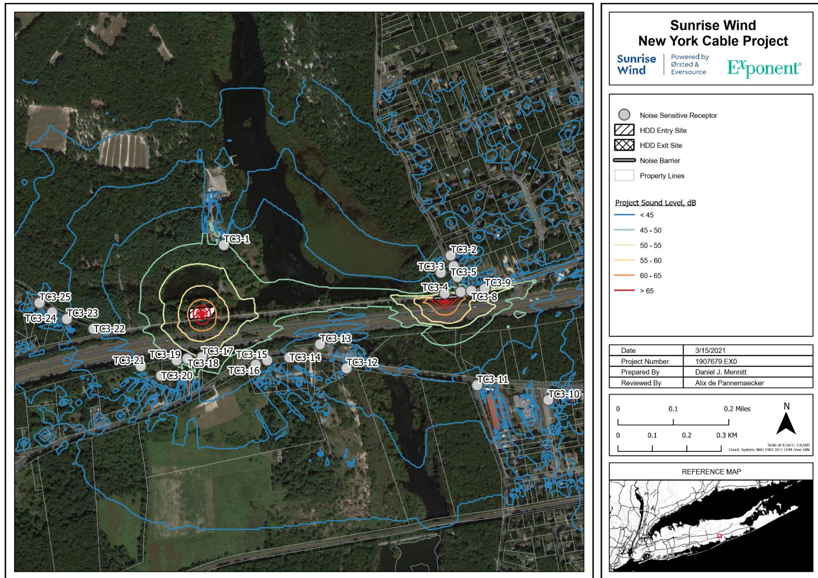
Revised Figure 15. TC3 HDD daytime construction noise contours.
